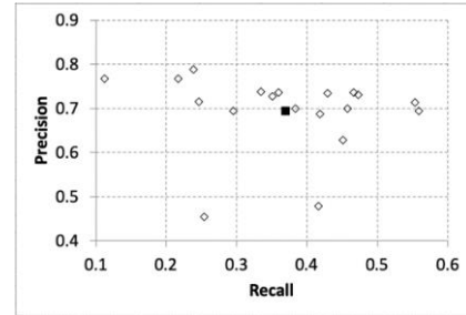
Figure 8. Performance evaluation of the proposed method over nineteen test subjects demonstrated via precision-recall scatter matrix. Average over all subjects is marked with a square.
